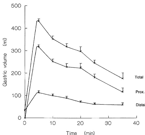
Figure 4. Proximal, distal, and total gastric volumes plotted against time to show the day-to-day variability of 1 healthy subject who was scanned on 6 consecutive days. Mean values and SEM are depicted, originating from data acquired by 3D ultrasonography by means of magnetic scanhead tracking.
